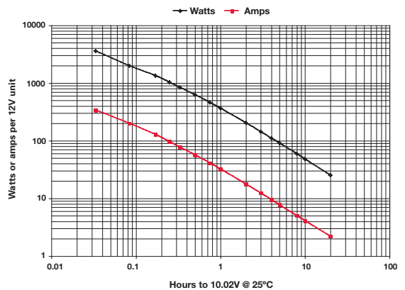
PC1200 performance data at 25°C, per 12V module
