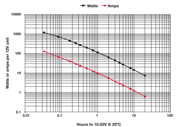
PC545 performance data at 25°C, per 12V module
