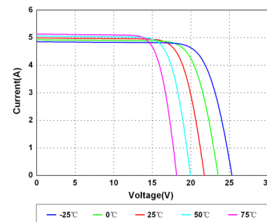
Current-Voltage Curves at Different Temperatures
