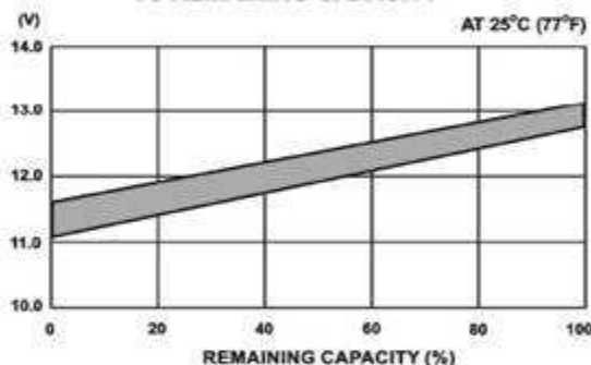
OPEN CIRCUIT VOLTAGE VS REMAINING CAPACITY
