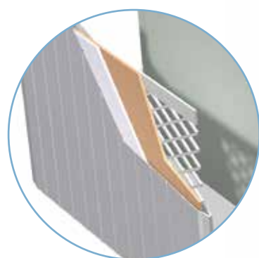
Positive plate: 3DX grid and advanced glass mat retainer covering active mass
